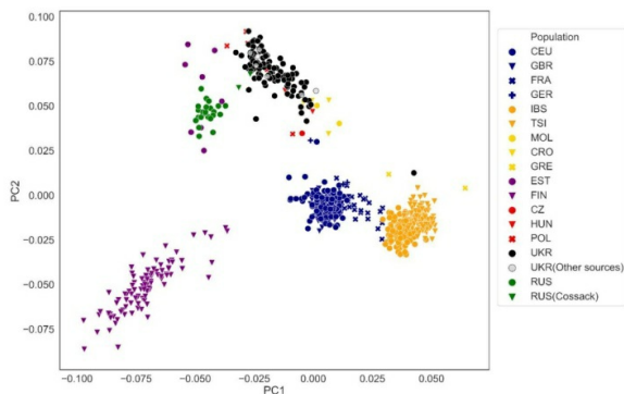
Figure 2: Principal component (PC) analysis of genetic merged dataset, containing European populations. Colors reflect ...
